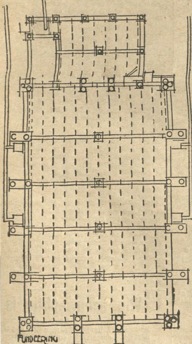
FUND. GROND
